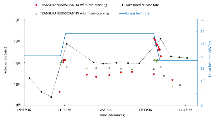
Fig. 13: ^{133}\text{Xe} release rate measured during the seventh power transient. The measurements (black dots) are compared against the TRANSURANUS/SCIANTIX calculation considering the burst release contribution from the micro-cracking (red dots) and neglecting it (green triangles).
