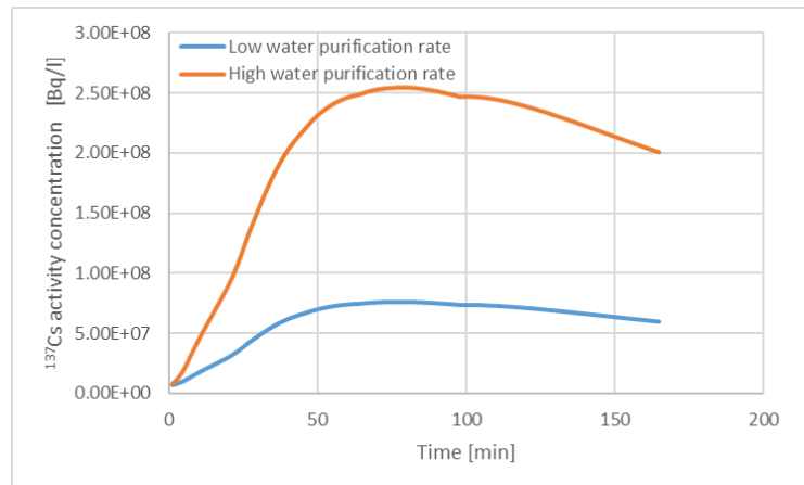
Fig. 44: Calculated ^{137}\text{Cs} activity concentration of the primary coolant during the collector cover opening event.
