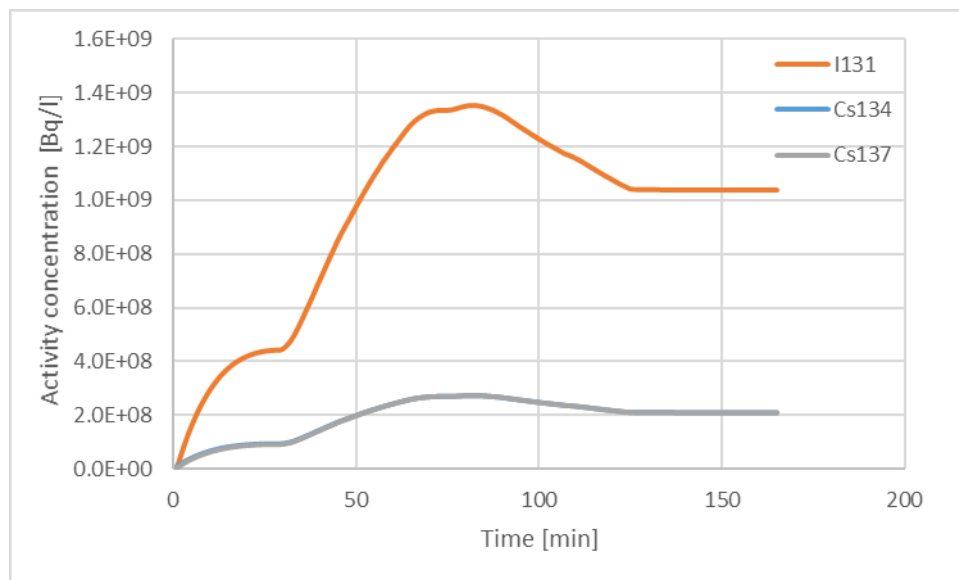
Fig. 37: ^{131}\text{I} , ^{134}\text{Cs} and ^{137}\text{Cs} corrected activity concentrations of the primary coolant during the break of 3 steam generator tube event ( ^{134}\text{Cs} and ^{137}\text{Cs} data are very close to each other and cannot be seen separately).
