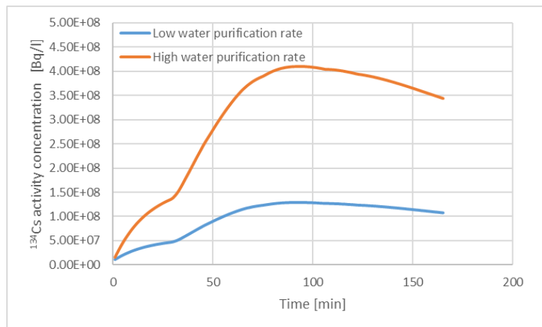
Fig. 35: Calculated ^{134}\text{Cs} activity concentration of the primary coolant during the break of 3 steam generator tube event.
