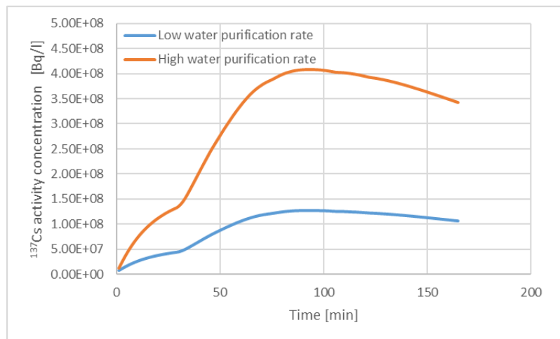
Fig. 36: Calculated ^{137}\text{Cs} activity concentration of the primary coolant during the break of 3 steam generator tube event.
