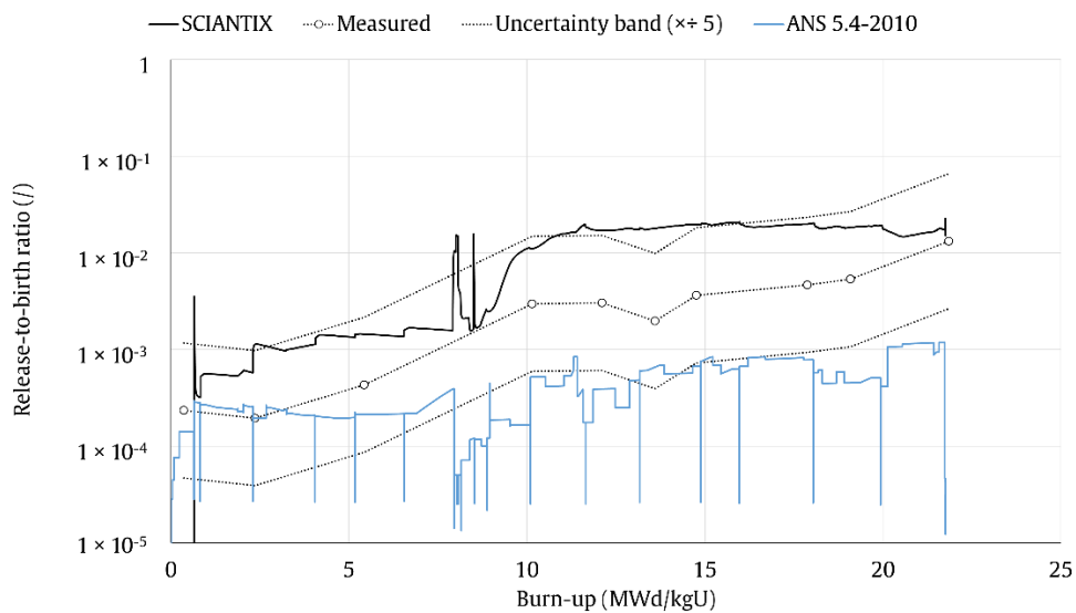
Fig. 3: Comparison of the release-to-birth ratio measured during the CONTACT 1 experiment (white dots) against the SCIENTIX prediction (black solid line) and the ANS 5.4-2010 prediction (blue line), for the short-lived ^{88}\text{Kr} .
