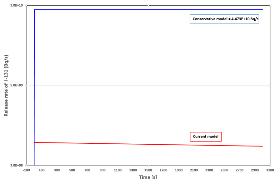
Fig. 54: Release activity of the ^{131}\text{I} into the RCS (scenario MSLB + 3 SGTR).
