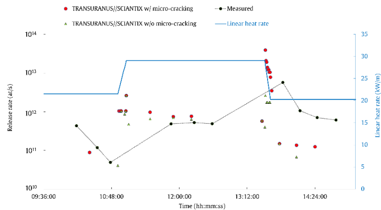
Fig. 12: ^{133}\text{Xe} release rate measured during the sixth power transient. The measurements (black dots) are compared against the TRANSURANUS/SCIANTIX calculation considering the burst release contribution from the micro-cracking (red dots) and neglecting it (green triangles).
