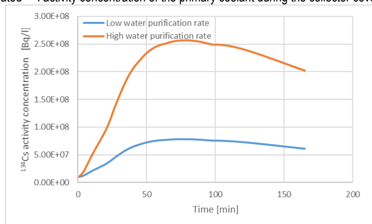
Fig. 43: Calculated ^{134}\text{Cs} activity concentration of the primary coolant during the collector cover opening event.
