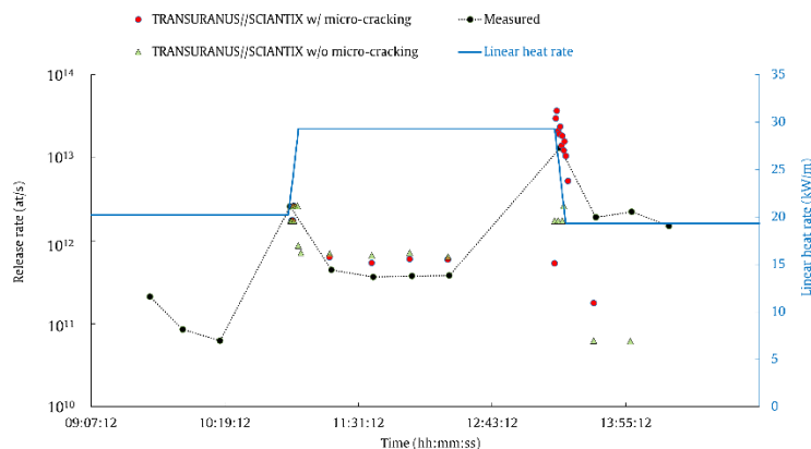
Fig. 11: ^{133}\text{Xe} release rate measured during the fifth power transient. The measurements (black dots) are compared against the TRANSURANUS/SCIANTIX calculation considering the burst release contribution from the micro-cracking (red dots) and neglecting it (green triangles).
