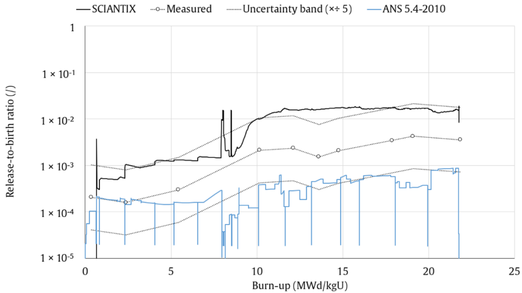
Fig. 2: Comparison of the release-to-birth ratio measured during the CONTACT 1 experiment (white dots) against the SCIENTIX prediction (black solid line) and the ANS 5.4-2010 prediction (blue line), for the short-lived ^{87}\text{Kr} .
