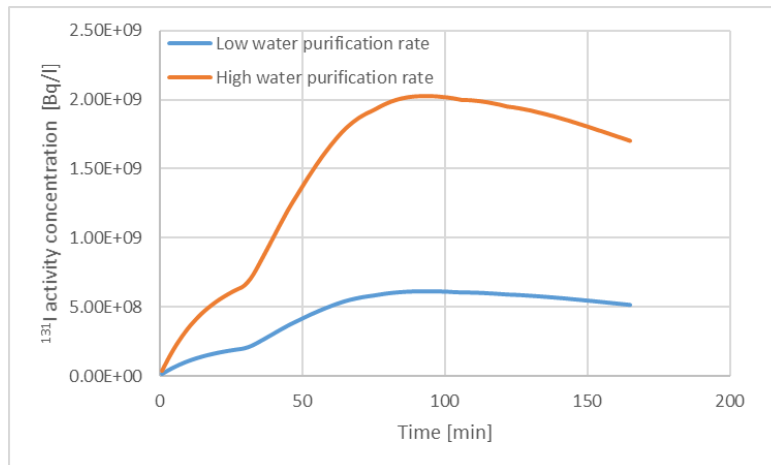
Fig. 34: Calculated ^{131}\text{I} activity concentration of the primary coolant during the break of 3 steam generator tube event.
