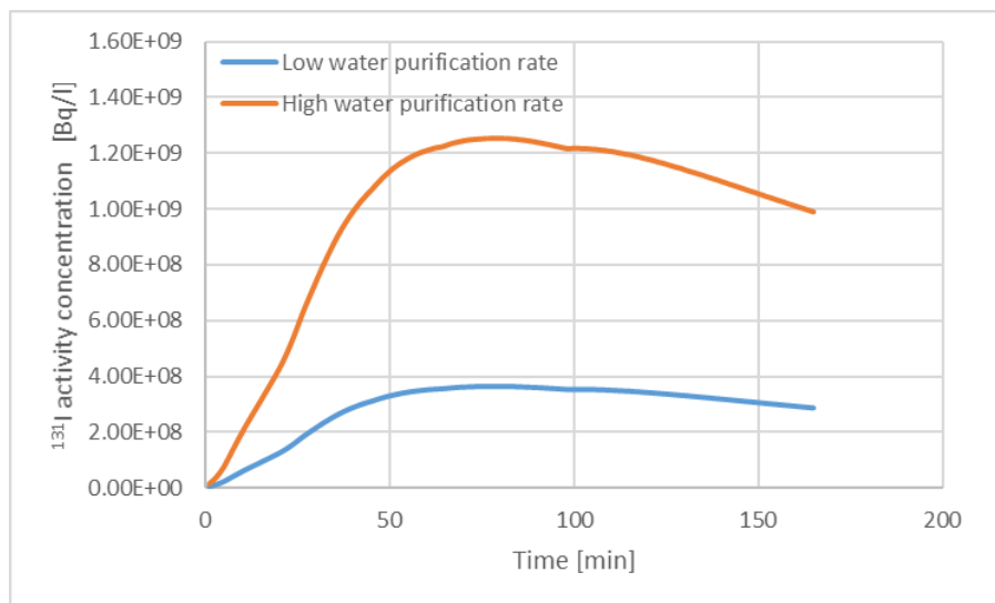
Fig. 42: Calculated ^{131}\text{I} activity concentration of the primary coolant during the collector cover opening event.
