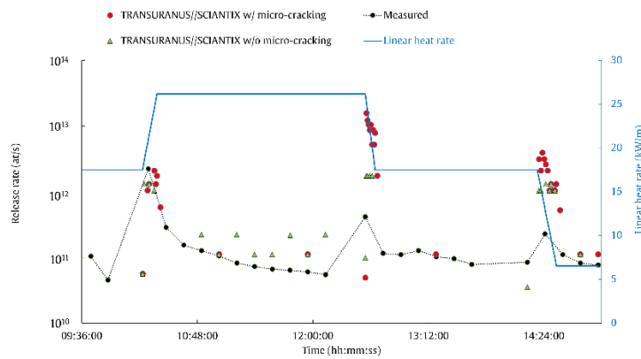
Fig. 16: ^{133}\text{Xe} release rate measured during the tenth power transient. The measurements (black dots) are compared against the TRANSURANUS/SCIANTIX calculation considering the burst release contribution from the micro-cracking (red dots) and neglecting it (green triangles).
