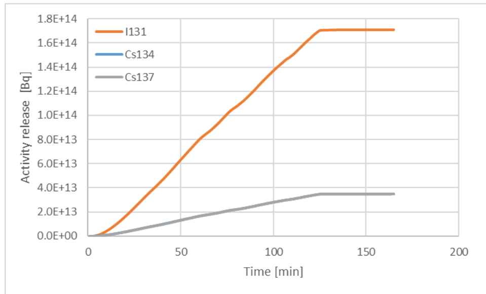
Fig. 38: ^{131}\text{I} , ^{134}\text{Cs} and ^{137}\text{Cs} activity release to the steam generator during the break of 3 steam generator tube event ( ^{134}\text{Cs} and ^{137}\text{Cs} data are very close to each other and cannot be seen separately).
