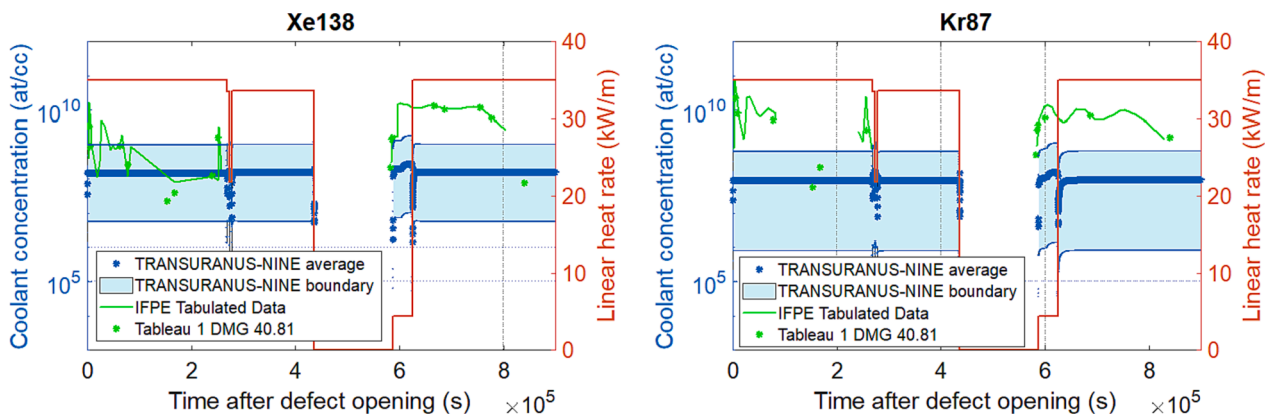
Fig. 6. Concentration of ^{138}\text{Xe} and ^{87}\text{Kr} in the coolant, after defect opening in the CRUSIFON1bis experiment. The blue dots represent the concentrations calculated with TRANSURANUS extended by NINE, inside the band of variation of calculated data (boundary). The green line represents the data reported in the IFPE documentation, interpolated from global activity measurements and the green dots represent experimental data from online measurements tabulated in the IFPE experimental report (i.e., Tableau DMG 40/81 (Harrer et al., 1980; Harrer et al., 1981)).
