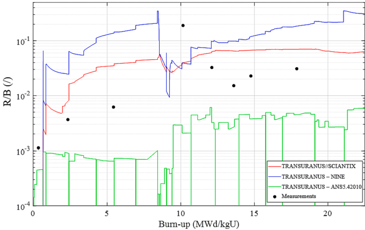
Fig. 4. Release-to-birth ratio of ^{133}\text{Xe} isotope, measured during the CONTACT1 experiment (data reported as black dots) along with code calculation results. The green line represents the prediction from ANS 5.4–2010 methodology, the semi-empirical algorithm recently implemented in TRANSURANUS (Turnbull and Beyer, 2010; Zullo et al., 2022c). The red line represents the calculation from the TRANSURANUS//SCIENTIX version (Zullo et al., 2022b; Zullo et al., 2022c). The blue line represents the calculation from the mechanistic TRANSURANUS fission gas behaviour model, extended at NINE to the radioactive isotopes as described in Section 2.2.
