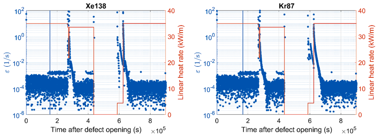
Fig. 5. Escape rate coefficients from defective cladding to primary coolant of ^{138}\text{Xe} and ^{87}\text{Kr} , after defect opening in the CRUSIFON1bis experiment (blue dots). The right y-axis reports the linear heat rate (red line). The vertical blue line at about 1.7 \times 10^5 s represents the time at which the steady-state condition is reached, from which stationary coolant concentrations were measured.
