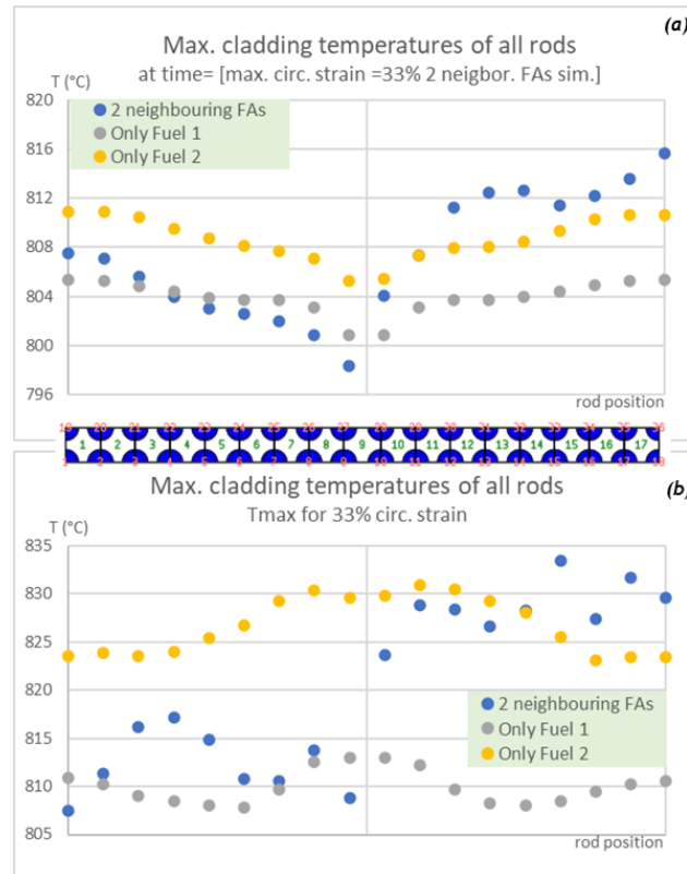
Figure 9: PCT for each rod obtained when max circumferential strain 33% is reached for first time by one rod (a) PCT for each rod when rod circumferential strain is 33% (b) PCT for each rod when rod circumferential strain is 33%
