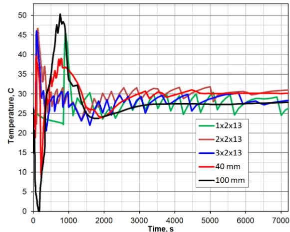
Figure 30: Evolution of the margin before boiling in primary (dT s ) during PRISE in VVER-1000 with the automatic accident control algorithm
