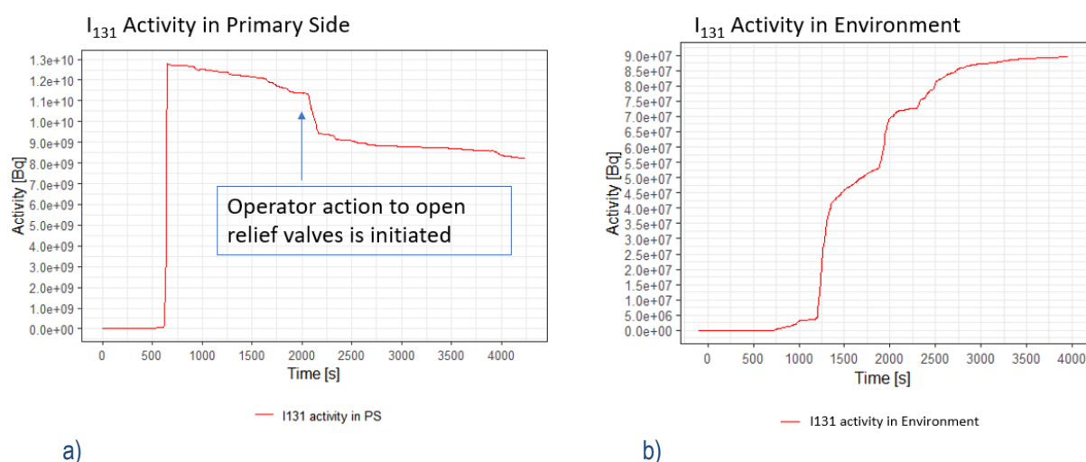
Figure 22: Preliminary transient calculation results of iodine activity in primary coolant (a) and environment (b) (FP transport model implemented in RELAP5-3D).
